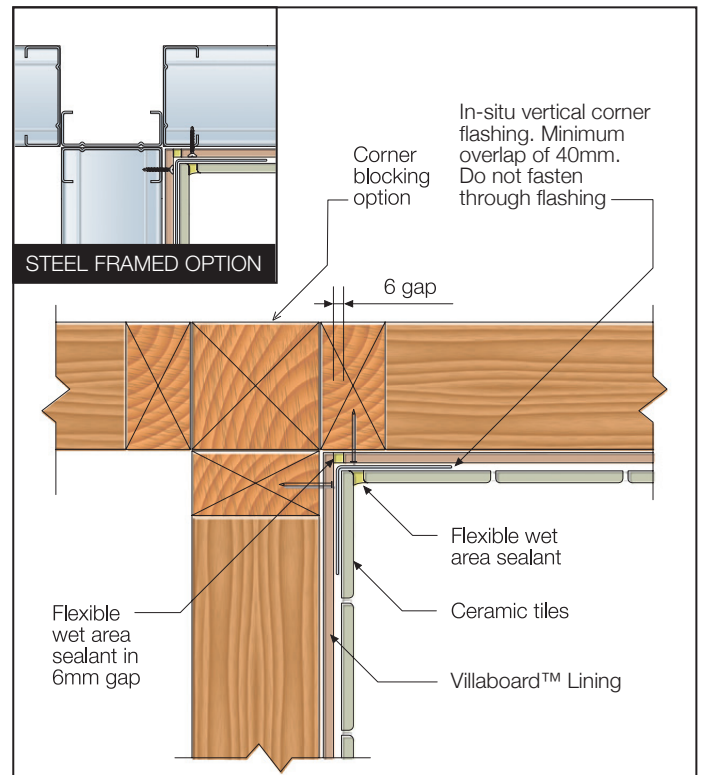
FIGURE 10 VERTICAL CORNER FLASHING FOR INTERNAL MEMBRANE - SHOWER RECESS
