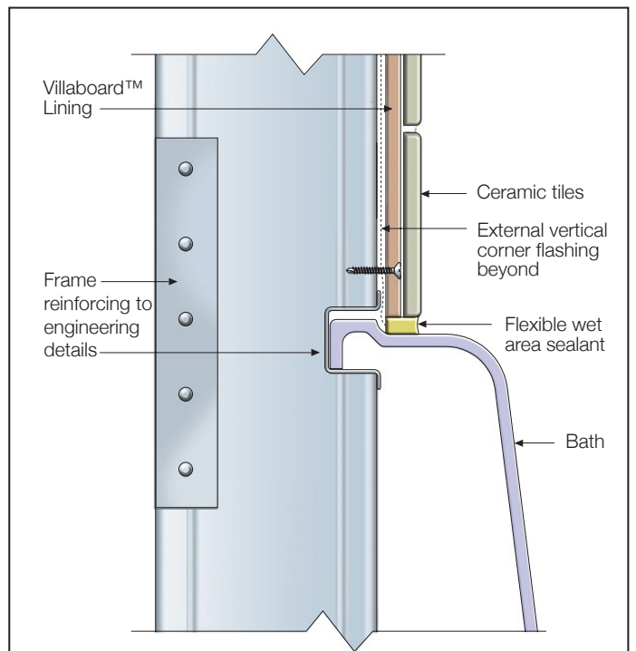
FIGURE 24B BATH EDGE DETAIL - VILLABOARD™ LINING TO BE FINISHED WITH TILES - STEEL FRAME
