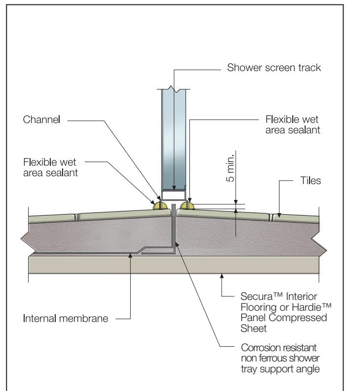
FIGURE 19 HOBLESS SHOWER
