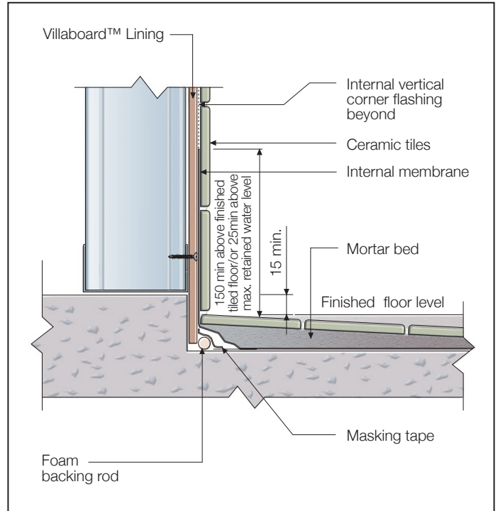
FIGURE 15B IN-SITU APPLIED INTERNAL MEMBRANE AT STEP-DOWN - STEEL FRAME OPTION
