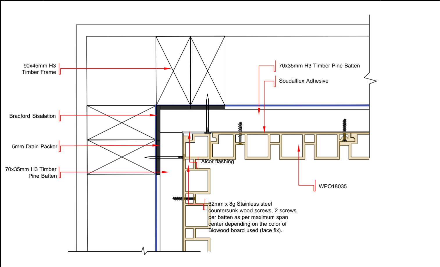
DWG - 05 PLAN VIEW OF INTERNAL CORNER DETAIL OF VERTICAL LAID BIOWOOD CLADDING - WPO18035 SCALE 1:3 @ A4
