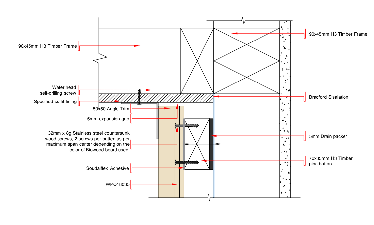
DWG - 11 SECTION VIEW OF CLADDING TO SOFFIT DETAIL OF VERTICAL LAID BIOWOOD CLADDING - WPO18035 SCALE 1:2.5 @ A4
