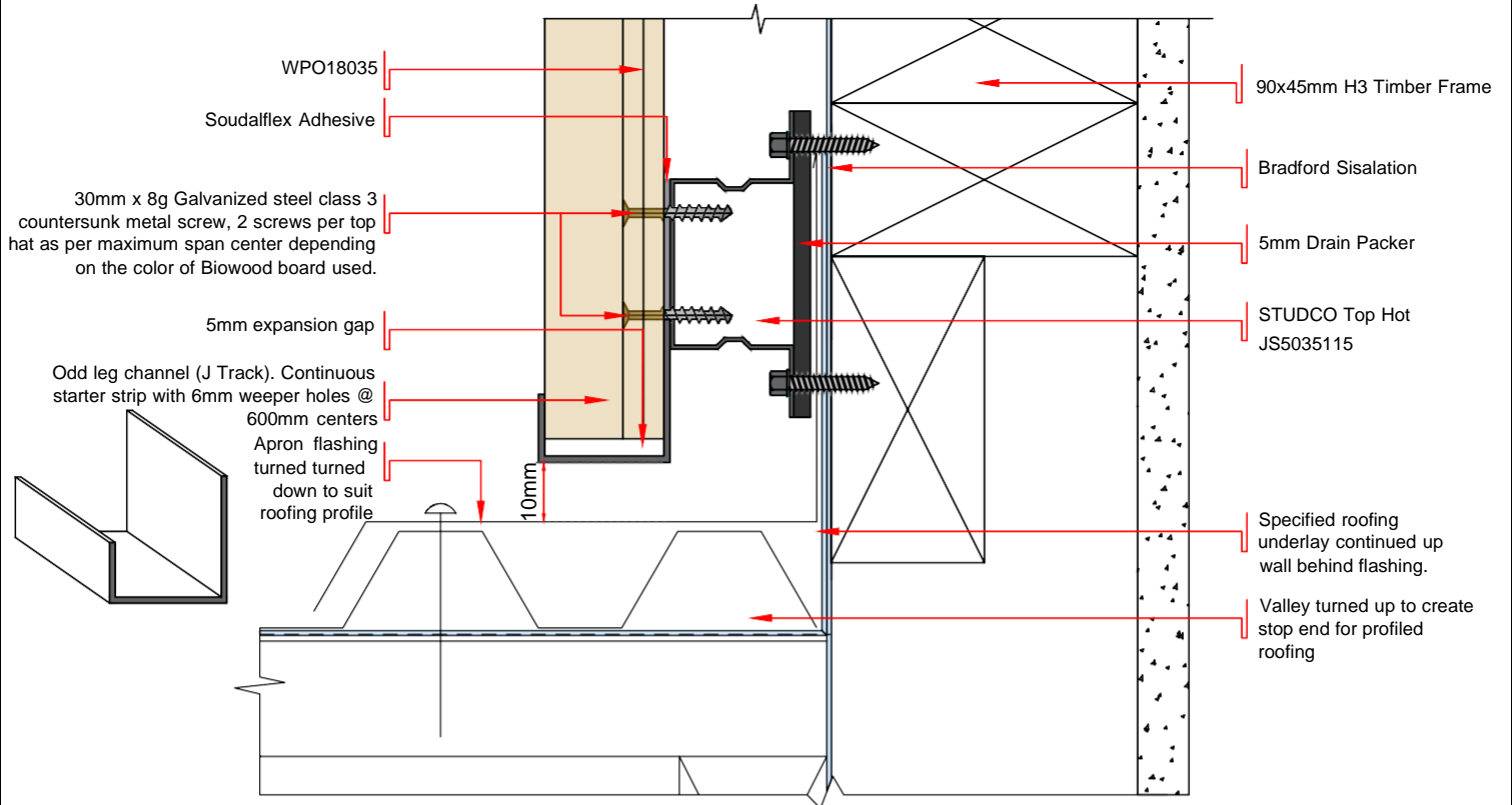
DWG - 10 SECTION VIEW OF PARALLEL APRON DETAIL OF VERTICAL LAID BIOWOOD CLADDING - WPO18035
