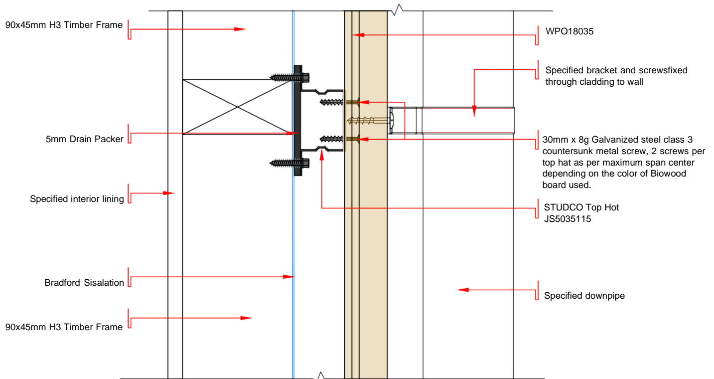
DWG - 13 SECTION VIEW OF DOWNPIPE FIXING DETAIL OF VERTICAL LAID BIOWOOD CLADDING - WPO18035 SCALE 1:3 @ A4
