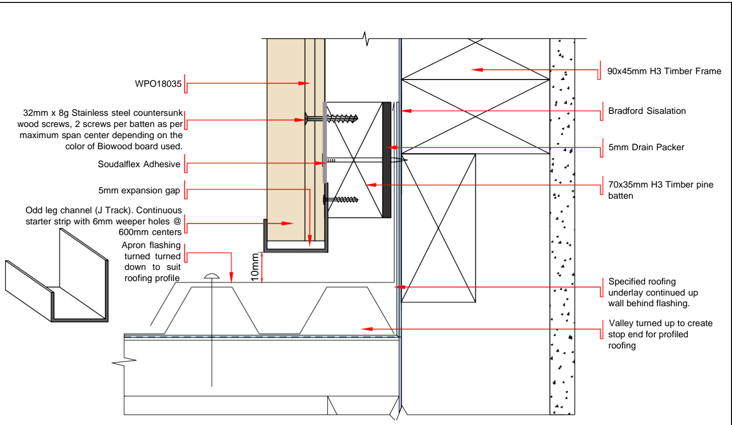
DWG - 10 SECTION VIEW OF PARALLEL APRON DETAIL OF VERTICAL LAID BIOWOOD CLADDING - WPO18035 SCALE 1:2.2 @ A4
