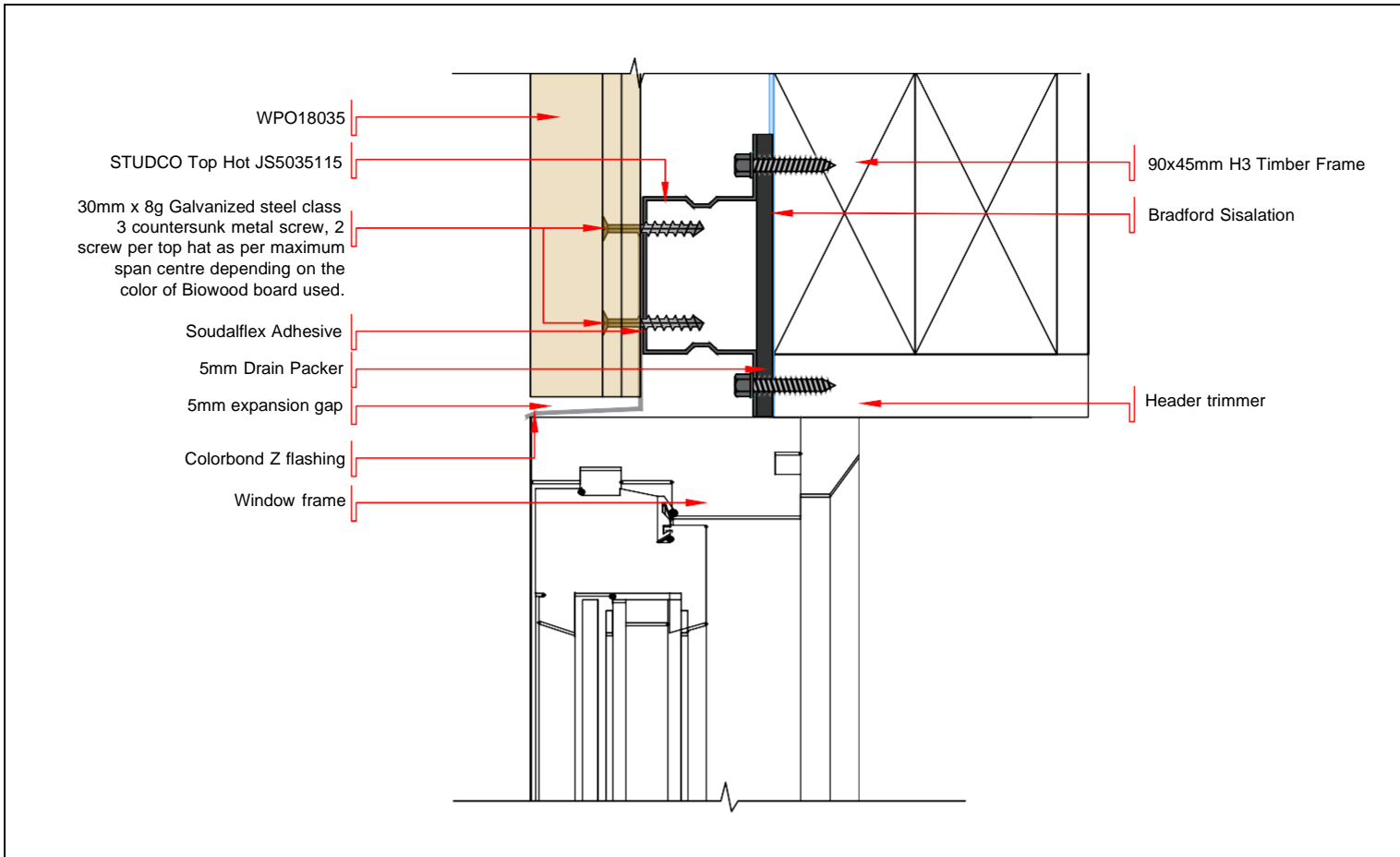
DWG - 06 SECTION VIEW OF WINDOW HEAD DETAIL OF VERTICAL LAID BIOWOOD CLADDING - WPO18035 SCALE 1:2.2 @ A4
