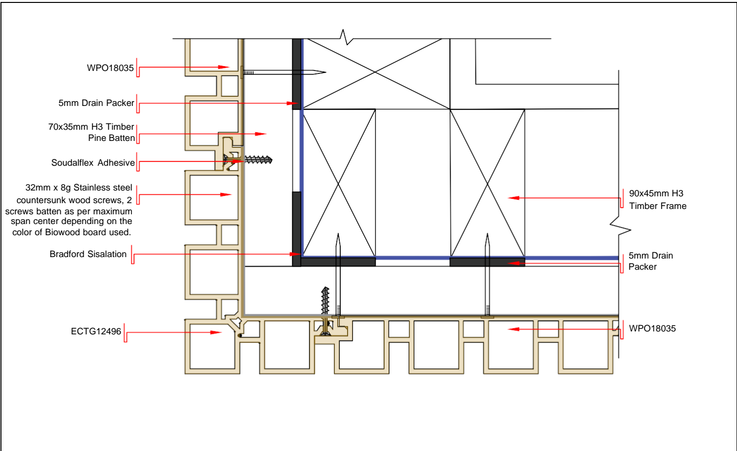
DWG - 04 PLAN VIEW OF EXTERNAL CORNER DETAIL OF VERTICAL LAID BIOWOOD CLADDING - WPO18035 SCALE 1:2.2 @ A4
