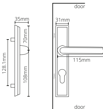
HANDLE DIMENSIONS
