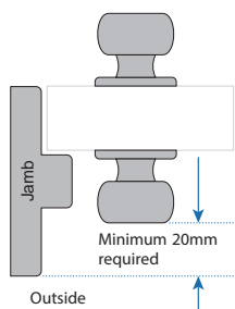
HANDLE DIMENSIONS
