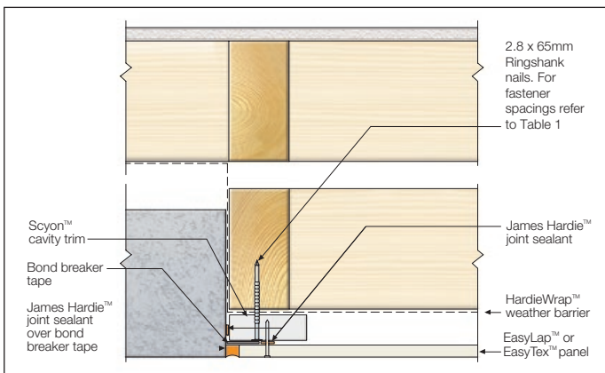
FIGURE 16 ABUTMENT DETAIL
