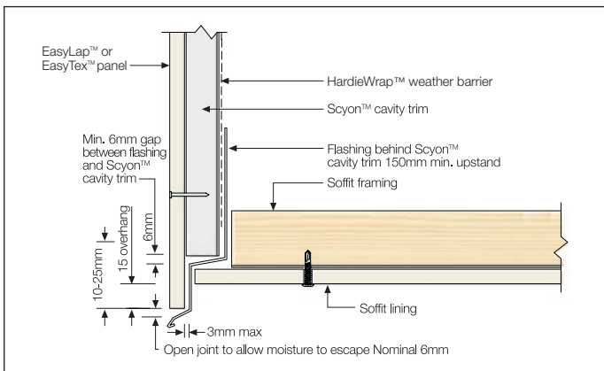
FIGURE 18 FACADE/SOFFIT JUNCTION
