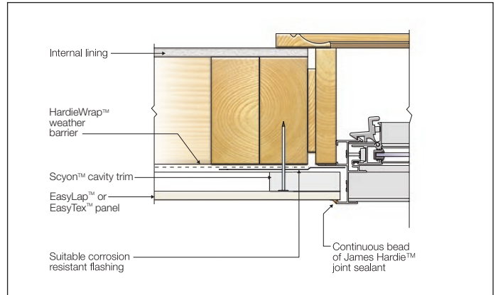
FIGURE 25 WINDOW JAMB - CAVITY TRIM
