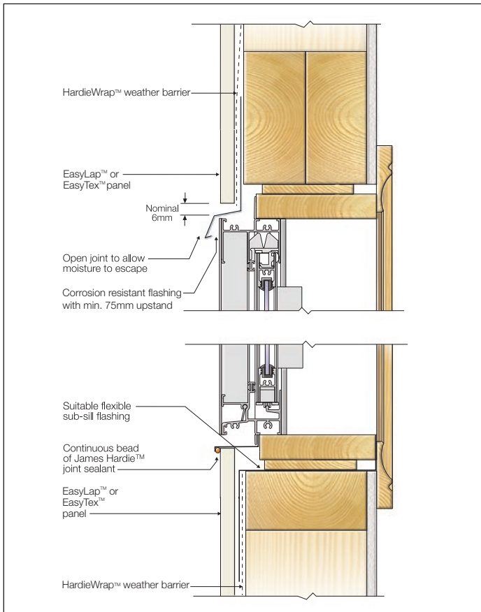
FIGURE 12 WINDOW HEAD AND SILL - TRIM
