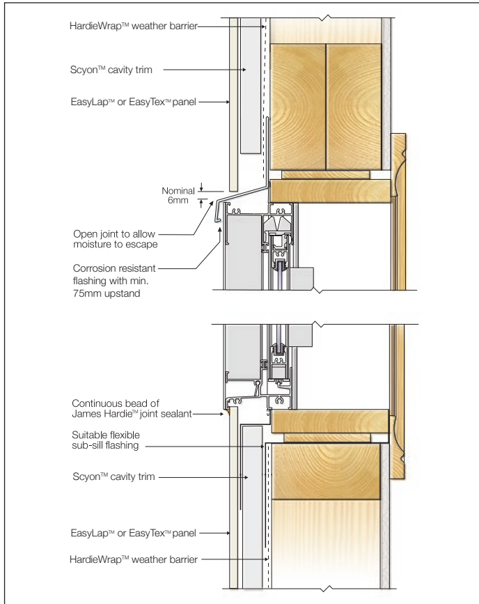
FIGURE 24 WINDOW HEAD AND SILL - CAVITY TRIM
