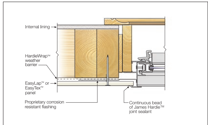
FIGURE 13 WINDOW JAMB - TRIM
