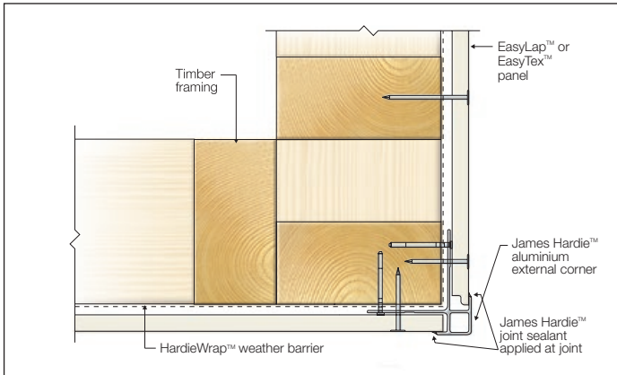
FIGURE 8 ALUMINIUM BOX CORNER OPTION
