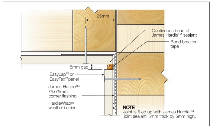
FIGURE 11 SEALANT FILL OPTION
