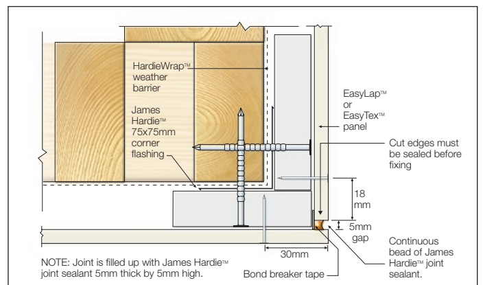
FIGURE 21 SEALANT FILL OPTION - CAVITY TRIM
