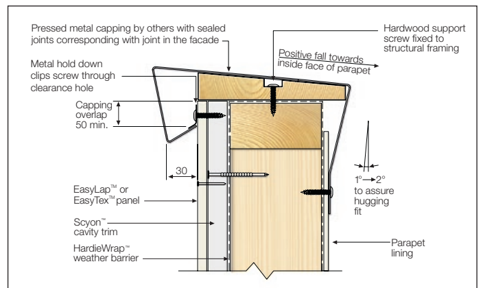
FIGURE 17 PARAPET CAPPING DETAIL
