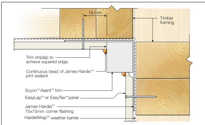
FIGURE 10 TRIM CORNER OPTION
