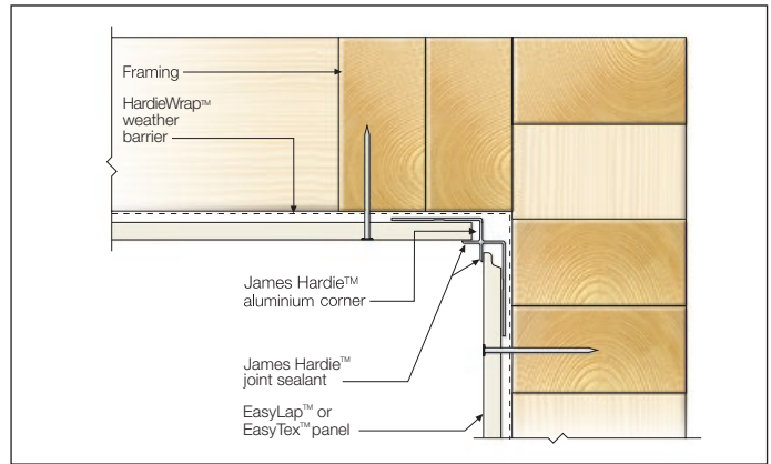
FIGURE 9 ALUMINIUM CORNER DETAIL
