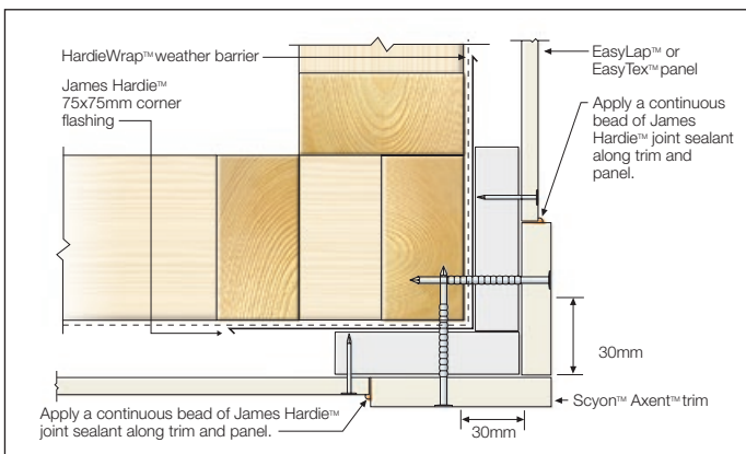
FIGURE 20 TRIM CORNER OPTION - CAVITY TRIM
