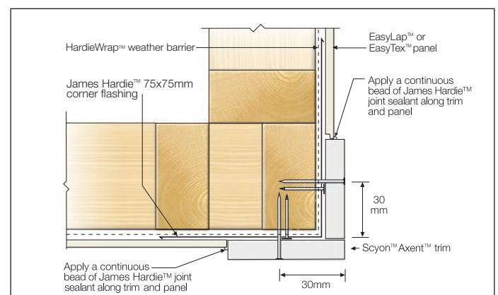
FIGURE 7 TRIM CORNER OPTION
