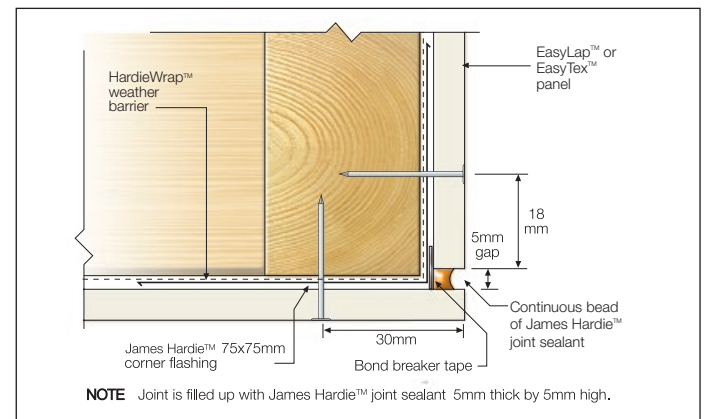
FIGURE 6 SEALANT FILL OPTION
