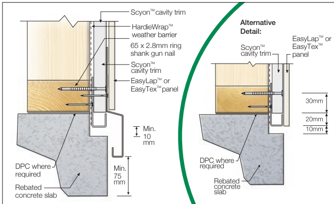
FIGURE 14 ALTERNATIVE SLAB EDGE DETAILS
