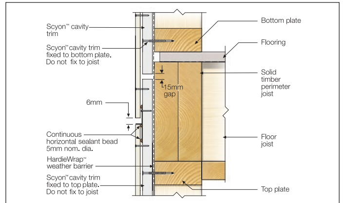
FIGURE 15 FLOOR LEVEL JUNCTION
