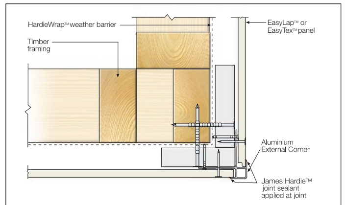
FIGURE 19 ALUMINIUM BOX CORNER OPTION - CAVITY TRIM
