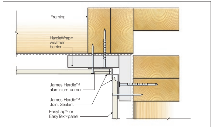
FIGURE 23 ALUMINIUM CORNER DETAIL - CAVITY TRIM
