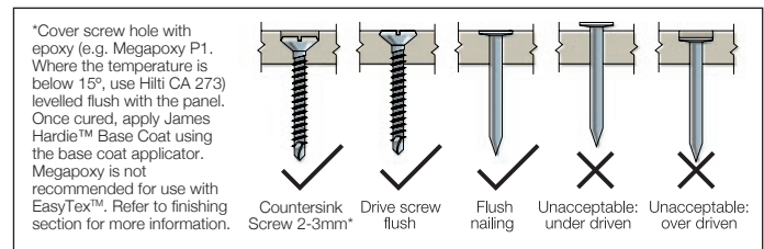
FIGURE 1 NAIL FASTENER DEPTH
