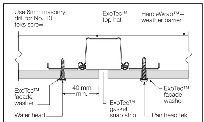
FIGURE 18 EXPOSED HEAD FASTENER DETAIL
