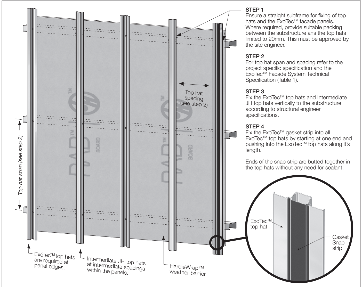
FIGURE 7 TOP HAT INSTALLATION
