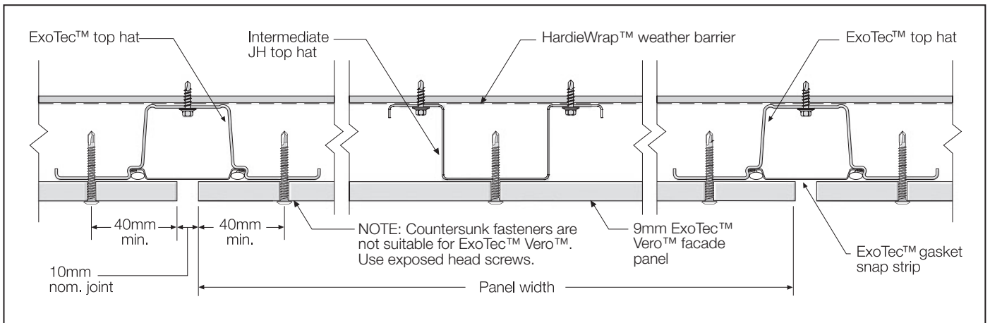
FIGURE 9 TOP HAT AND PANEL FIXING DETAIL FOR EXOTEC™ VERO™ PANELS
