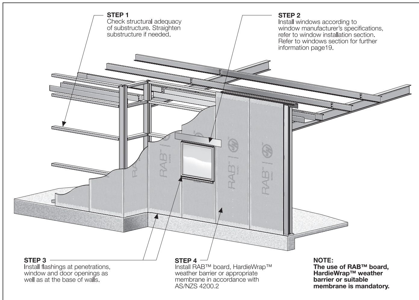
FIGURE 2 PREPARATION OF SUB-STRUCTURE
