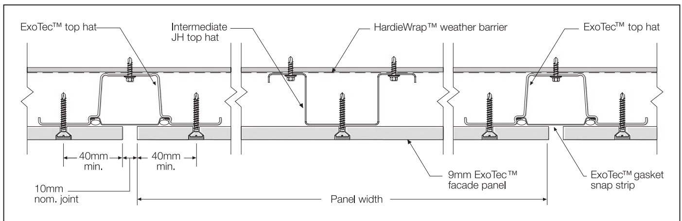
FIGURE 9 TOP HAT AND PANEL FIXING DETAIL FOR EXOTEC™ PANELS
