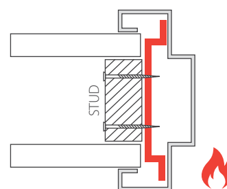
TOP HAT FIXING (CONCEALED EDGE OF WALL)
