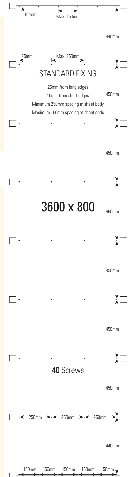
Figure 3. Fixing plan
