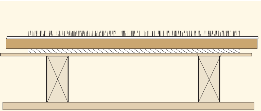
Floating Floor (over timber)
