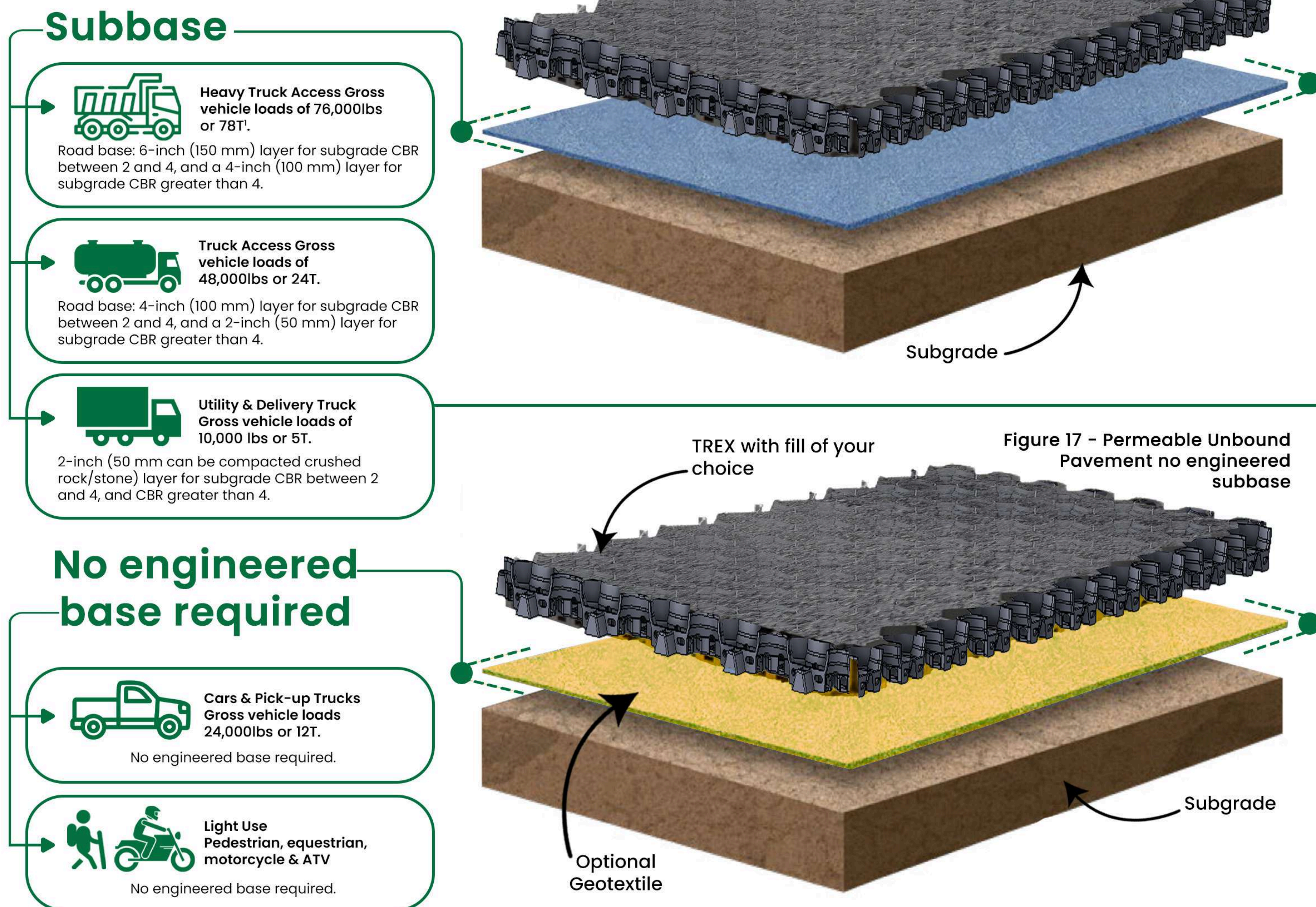
Figure 16 - Permeable Unbound Pavement with engineered subbase
