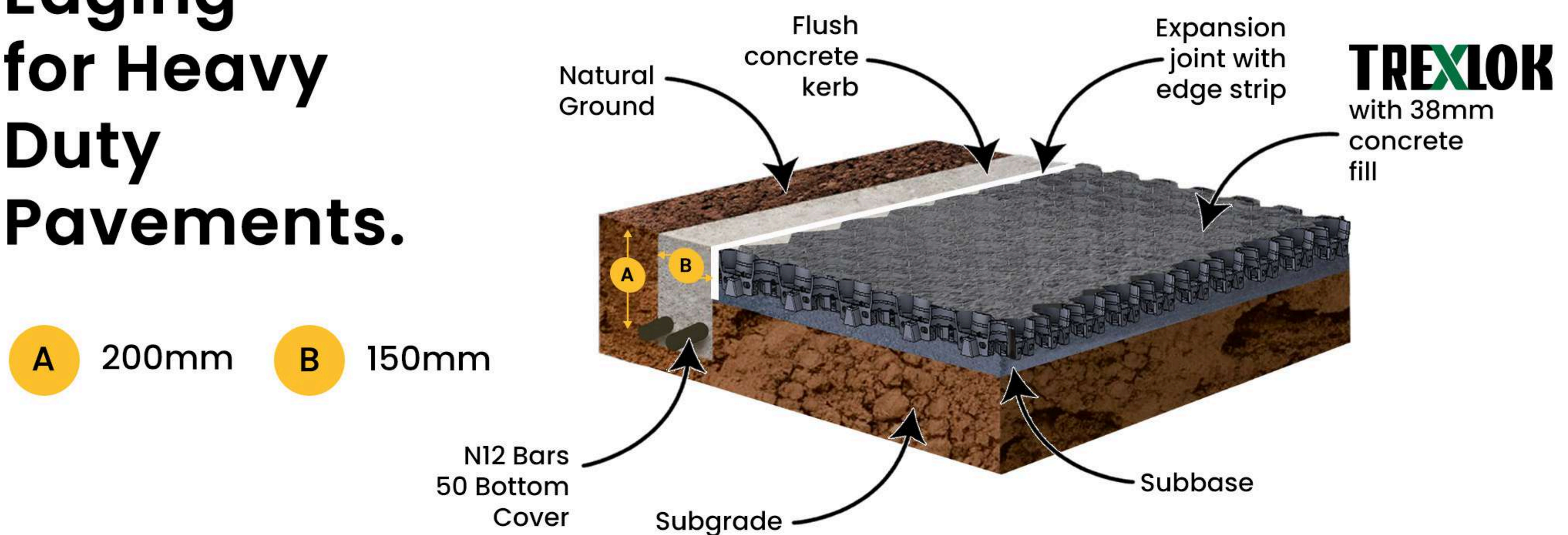
Figure 6 - For pavements requiring heavy duty applications that are subjected to heavy loads, edge reinforcement through a flush kerb is required.
