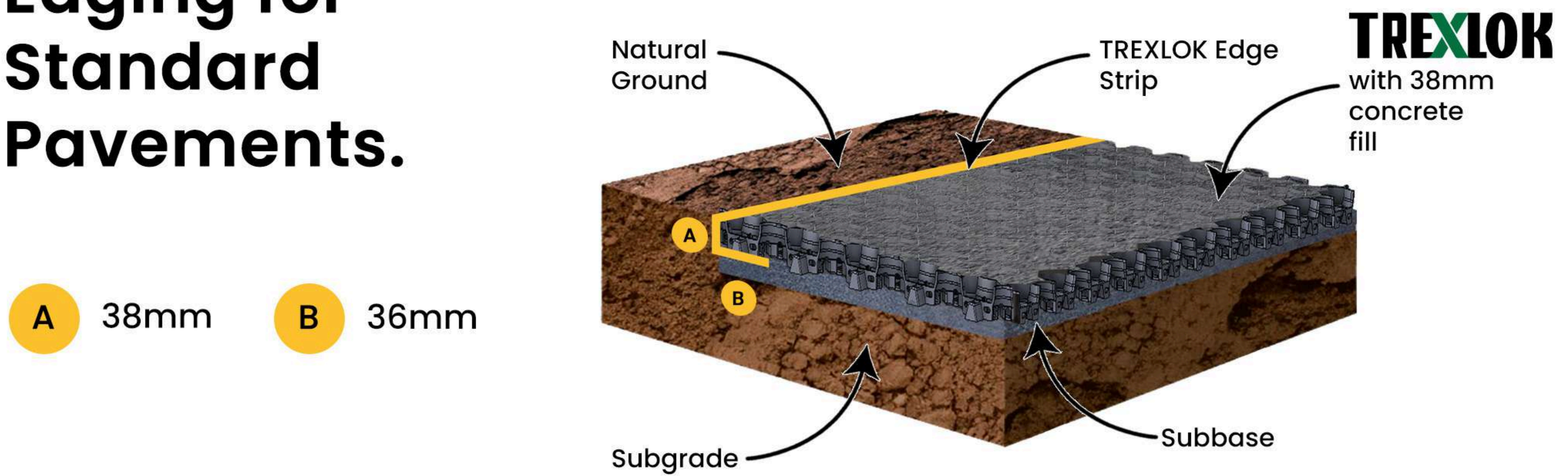
Figure 5 - Edging for standard pavements using "TREXLOK Edge Strip".
