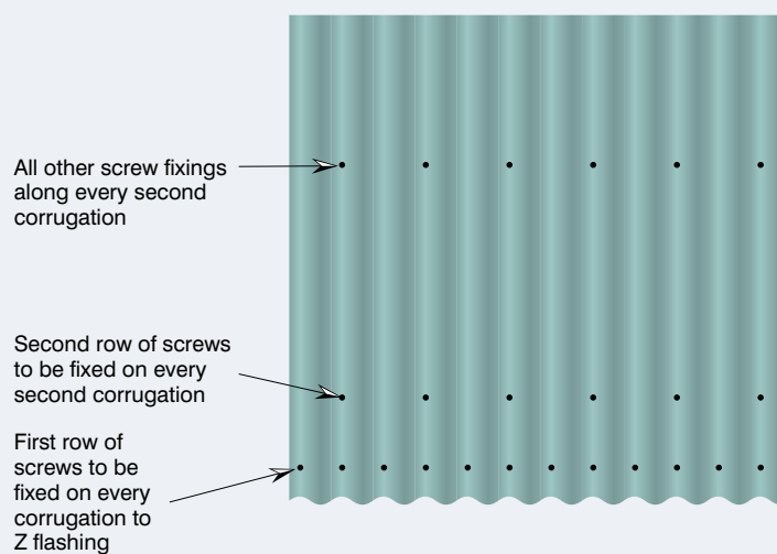
Diagram 3: Detail, Roof fixing requirements
