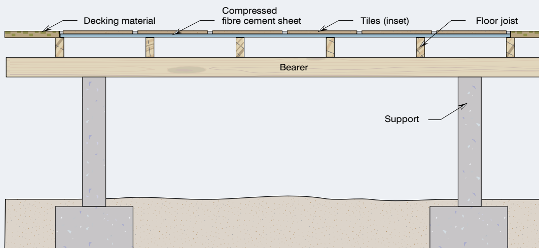
BAL-12.5 Diagram 2: Elevation View. Mixed material decking solution
